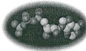
A molecule of ATP
